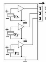
Electrical circuit
